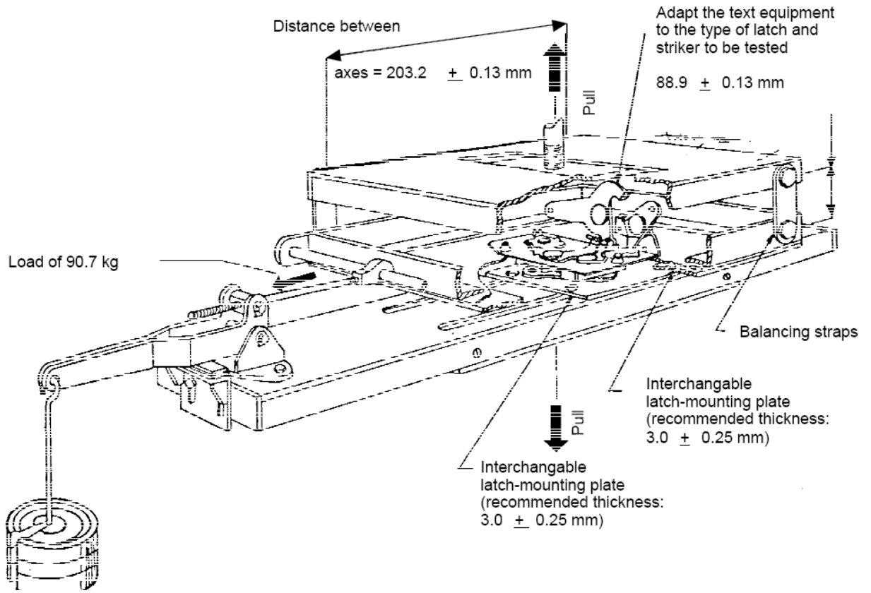
Fig. 2 - DOOR LATCH - TEST EQUIPMENT UNDER STATIC LOAD (LONGITUDINAL LOAD)
