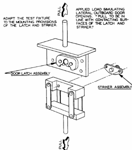
FIG. 3 - DOOR LATCHES - TEST EQUIPMENT UNDER STATIC LOAD (TRANSVERSE LOAD)
