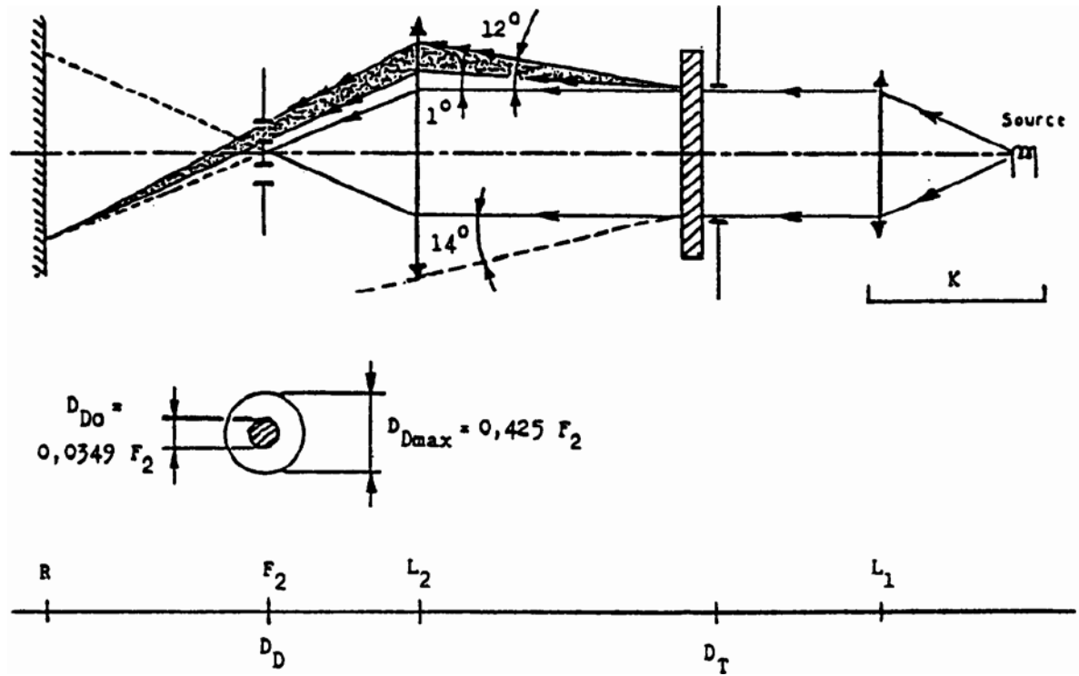
Optical setup for measurement of variations in diffusion and transmission
