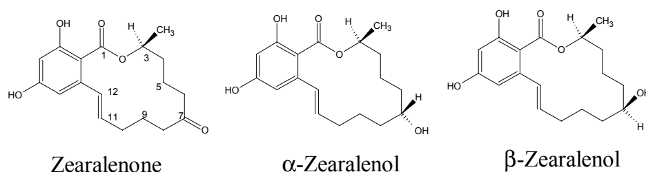
Figure 8: Chemical structures of zearalenone and primary metabolites
