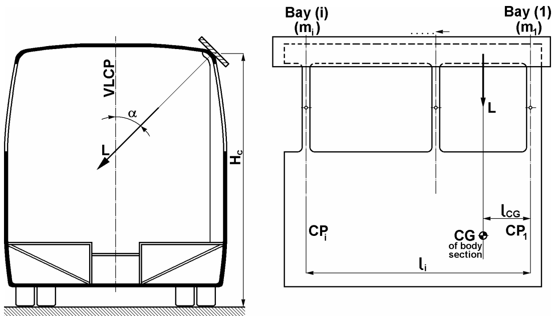
v)Figure A7.1 - Application of load to the body section
