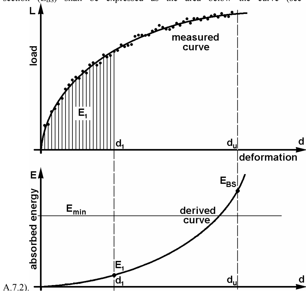
A.7.2). Figure A7.2 - Absorbed energy for the body section, derived from the measured load-deformation curve
