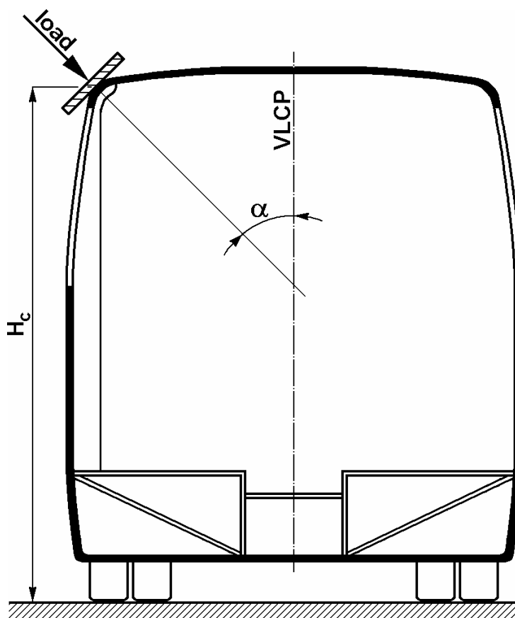
Figure A8. 2 - Load application to the superstructure
