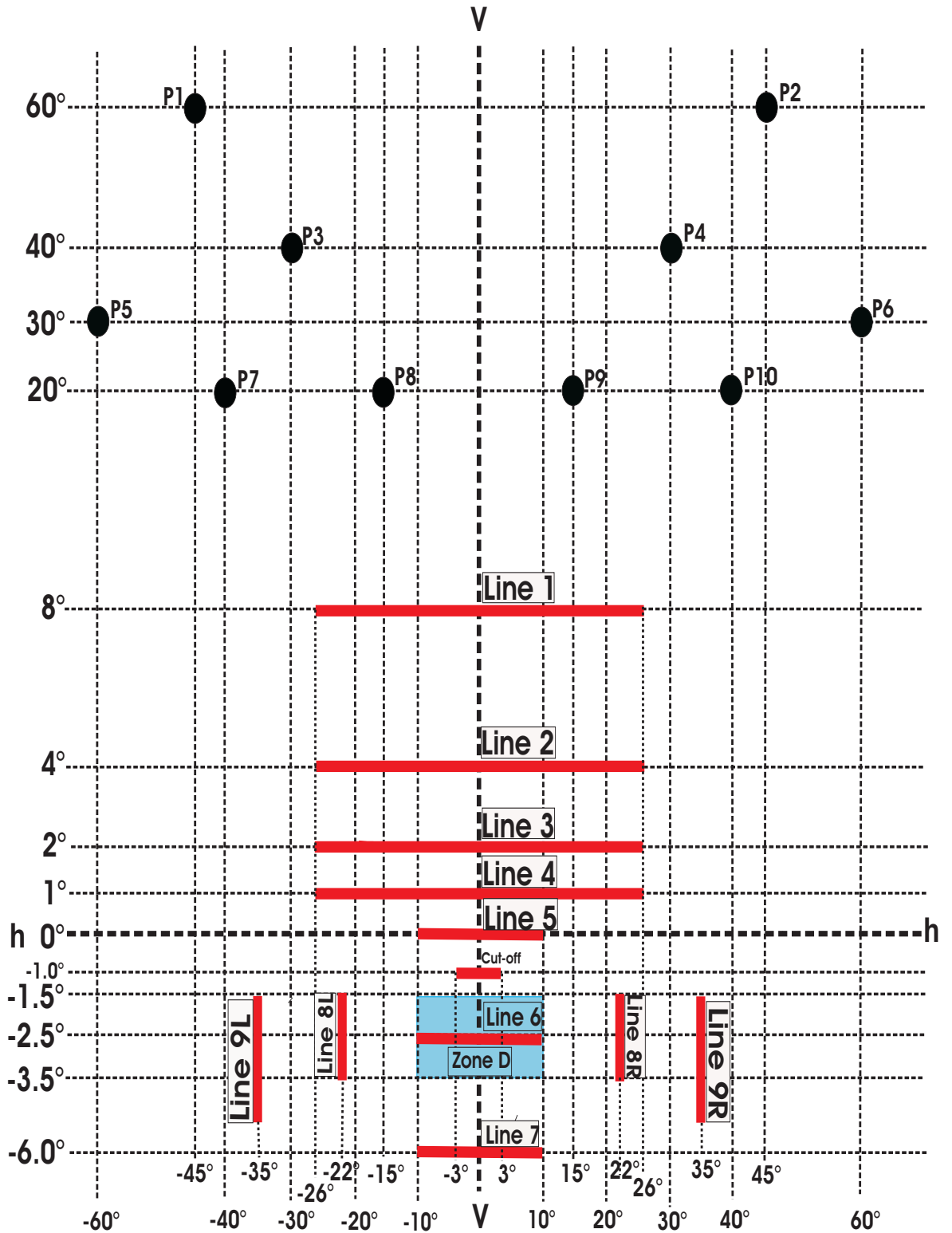
Figure 3: Light distribution of the Class F3 front fog lamp
