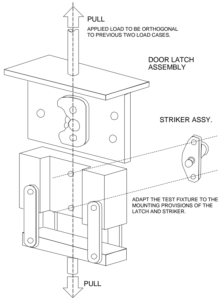
Figure 3-3 - Door Latch – Tensile Testing Fixture for Load Test Three (For doors that open in a vertical direction)
