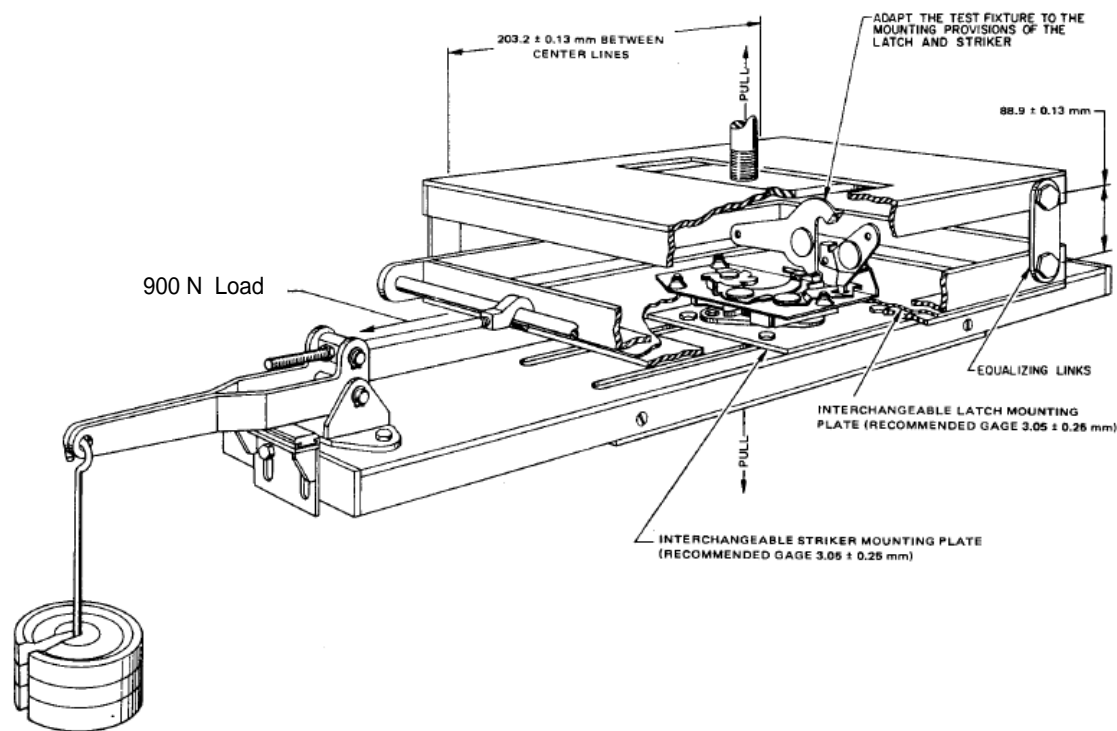
Figure 3-1 – Door Latch - Tensile Testing Fixture for Load Test One
