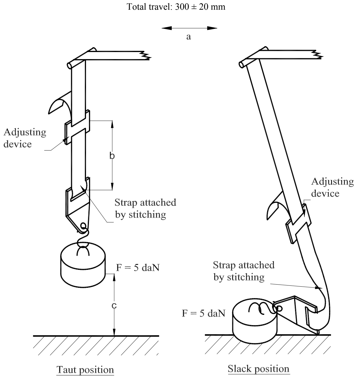
Figure 3: Type 3 procedure and micro-slip test
