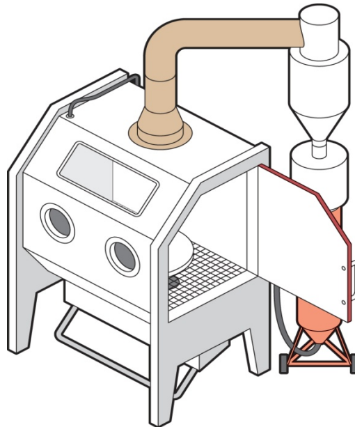
Figure 1: Blasting cabinet
