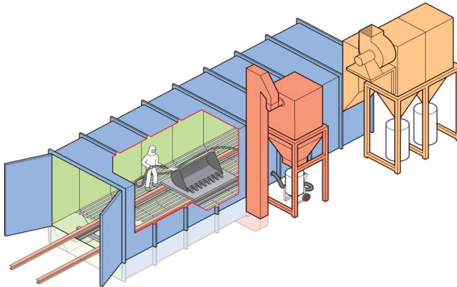
Figure 2: Blasting chamber
