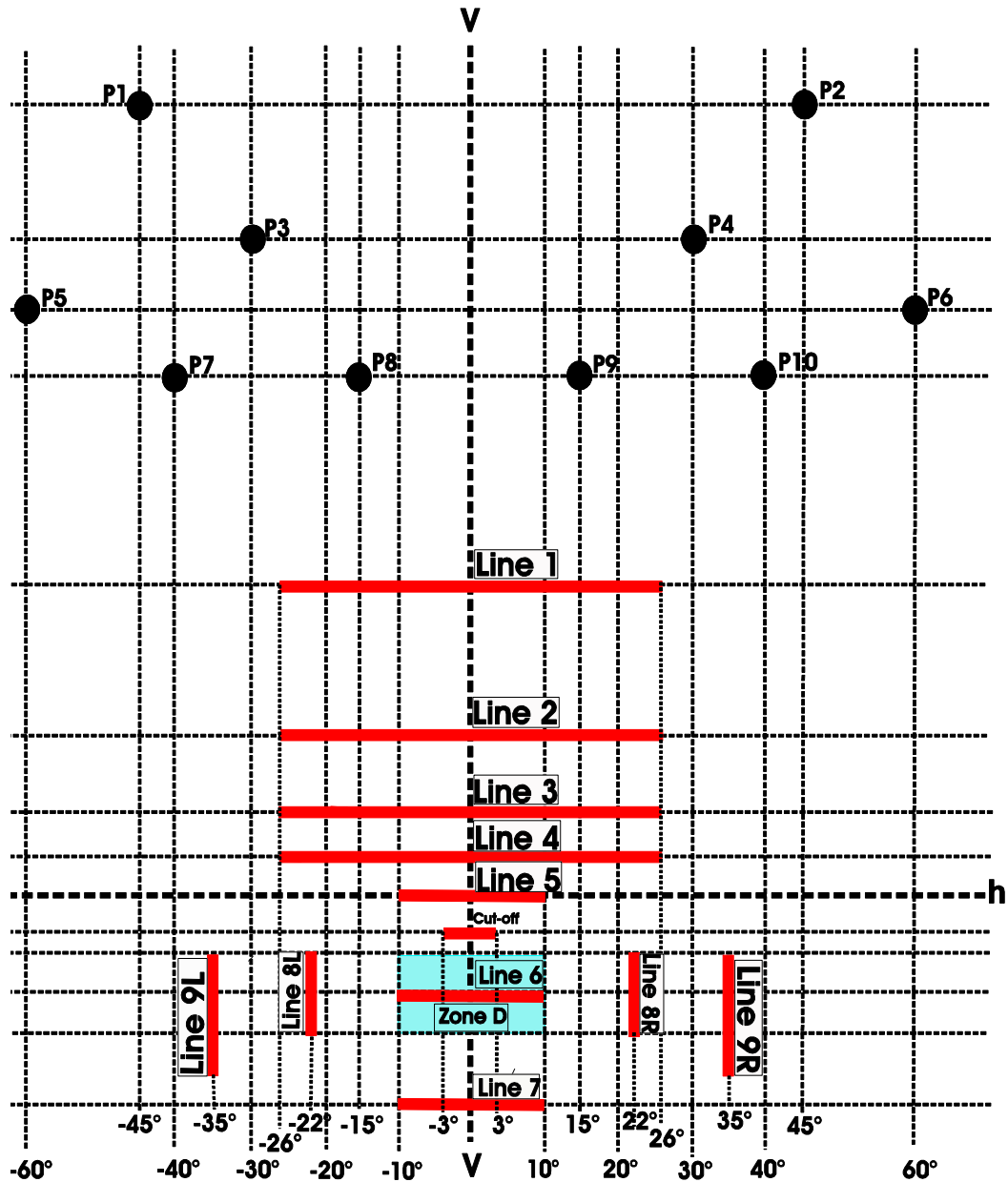
Figure 3 Light distribution of the Class F3 front fog lamp
