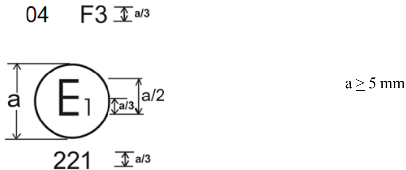
Figure 7 Examples of arrangements of approval marks for front fog lamps of Class "F3"
