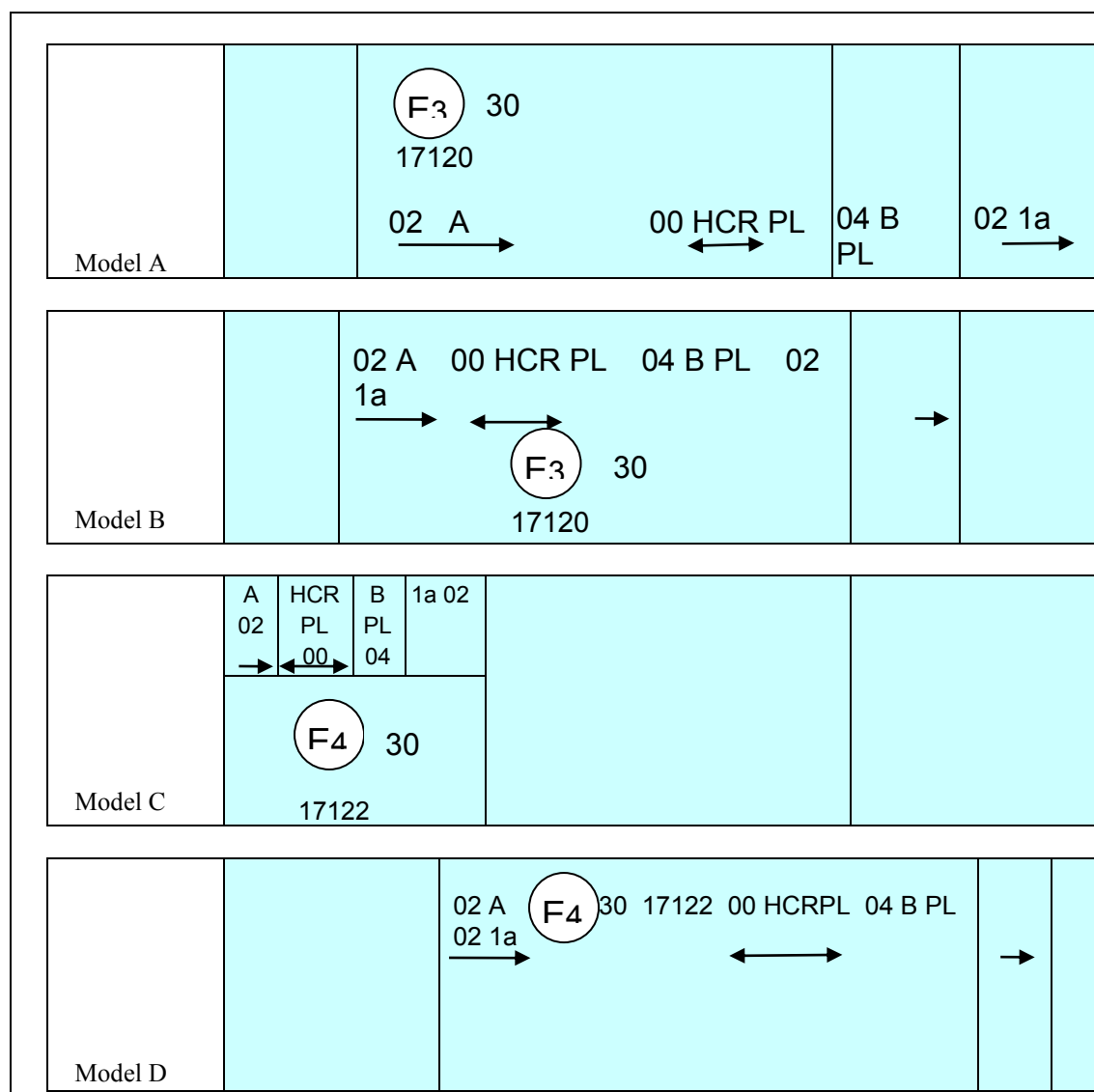
Figure 3 Examples of possible markings for grouped, combined or reciprocally incorporated lamps situated on the front of a vehicle
