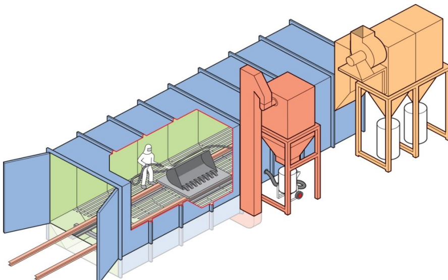
Figure 2 Blasting chamber
