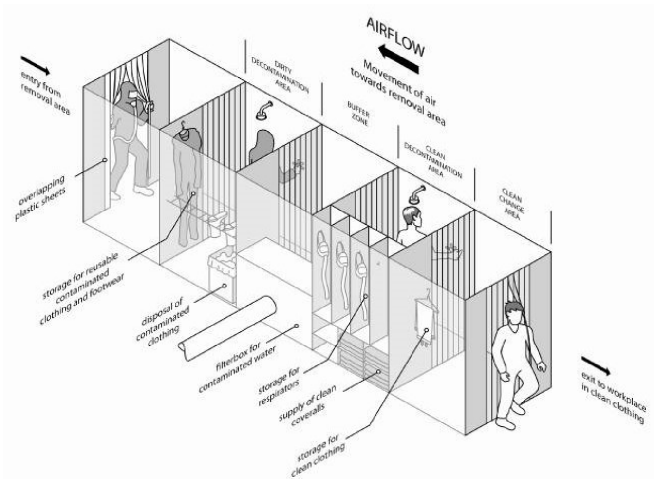
Figure 1 Decontamination unit
