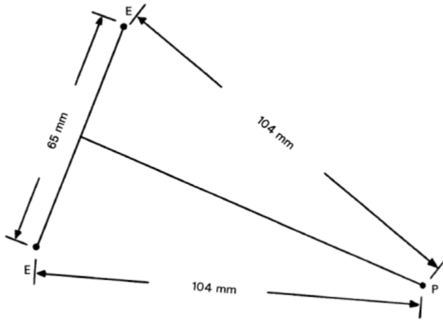
Figure 5 Dimensional diagram showing relative positions of E points and P points
