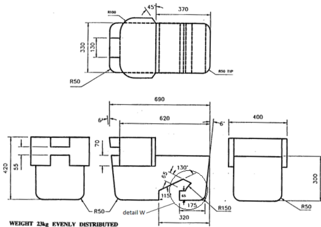
Figure 1 Specifications of the fixture (all dimensions in mm)
