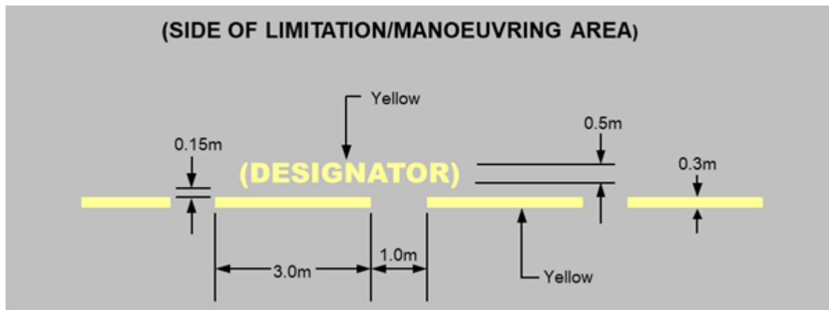
Figure 8.51 (2) Apron limit line with optional designer (shows matters)
