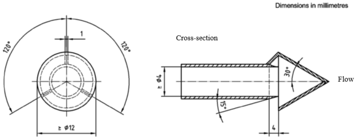
Figure 14 Scheme of hatted probe
