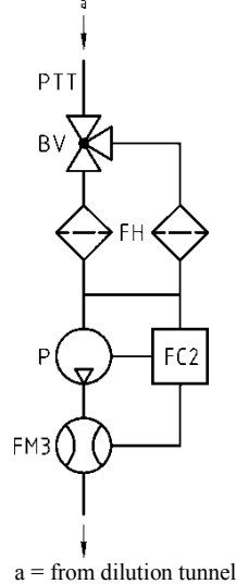
Figure 16 Scheme of particulate sampling system
