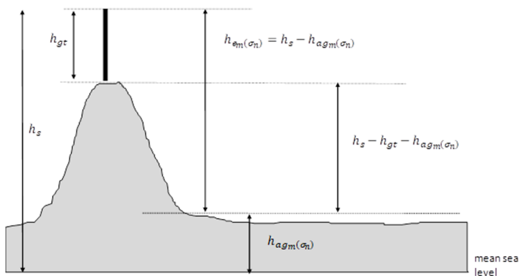
Diagram 1 Calculating effective antenna height
