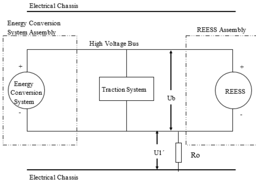
Figure 2 Measurement of U_1'
