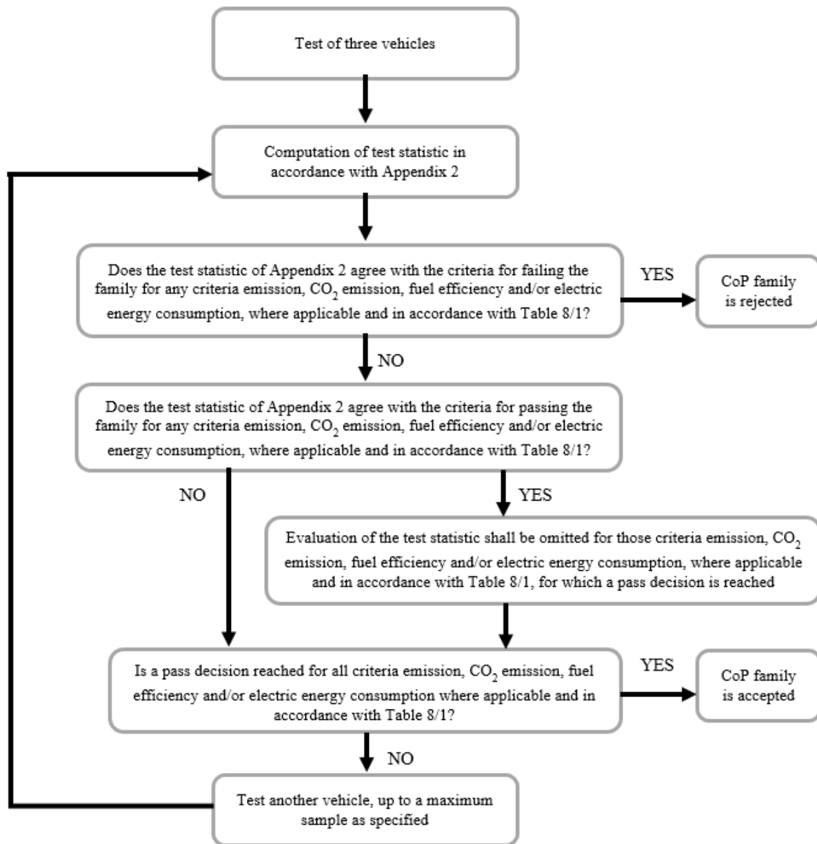
Figure 8/1 Flowchart of the CoP test
