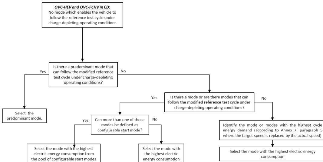
Figure A8.App6/1b OVC-HEV and OVC-FCHV (as applicable): CD Type 1 Test – Mode selectable switch
