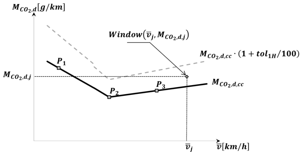
Vehicle CO 2 characteristic curve and tolerances for OVC-HEV vehicles
